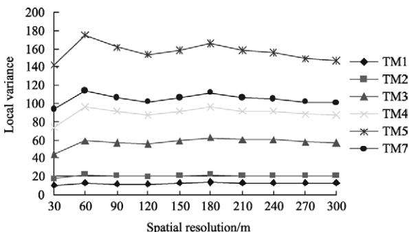
Fig. 8 Local variance as a function of resolution for the different TM band image
