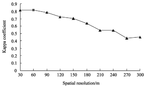
Fig. 7 Relationship between Kappa coefficient and resolution in the TM experiment
