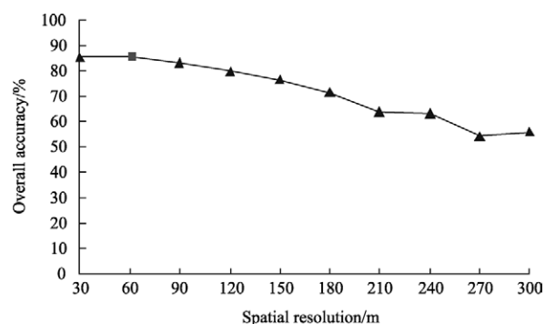
Fig. 6 Relationship between overall classification accuracy and resolution in the TM experiment
