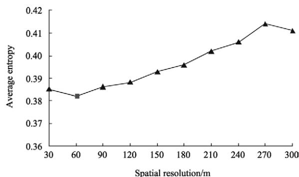
Fig. 5 Relationship between average entropy and resolution in the TM experiment
