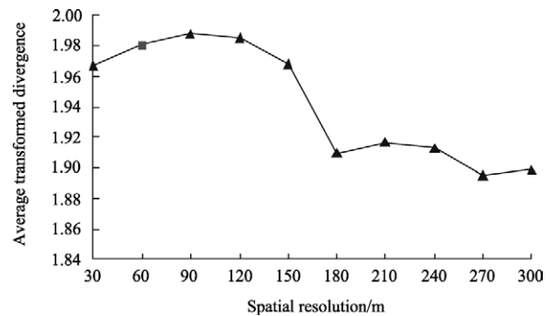
Fig. 10 Relationship between average transformed divergence and resolution in the TM experiment
